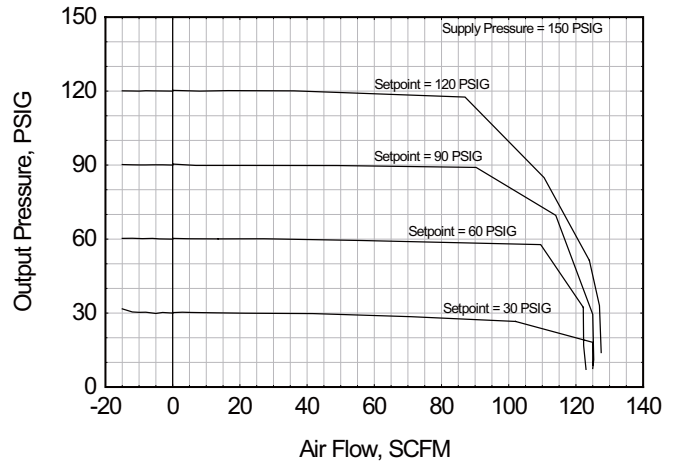
Flow Characteristics T9040-4074N4FJT Pressure Controller
