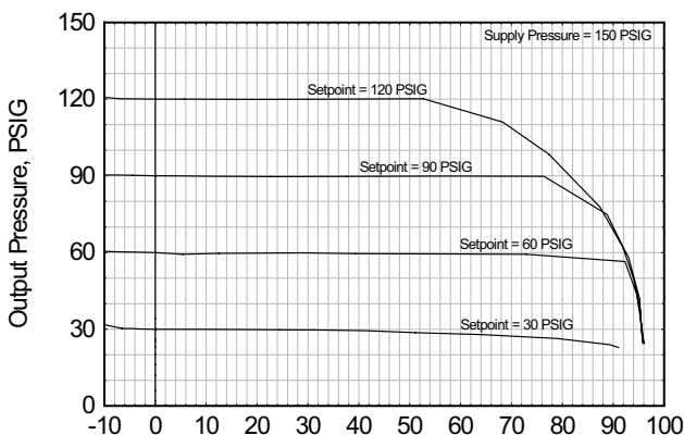
Flow Characteristics T9020-4072N4NFS Pressure Controller
