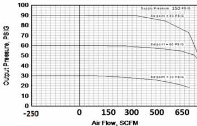
Flow Characteristics T9080-4078N4FNT Pressure Controller
